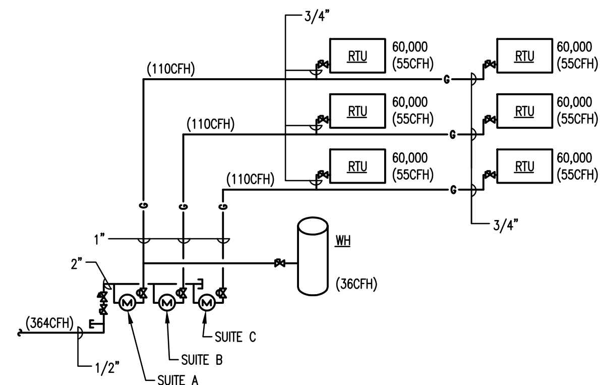
3 NATURAL GAS RISER SCALE: NOT TO SCALE
