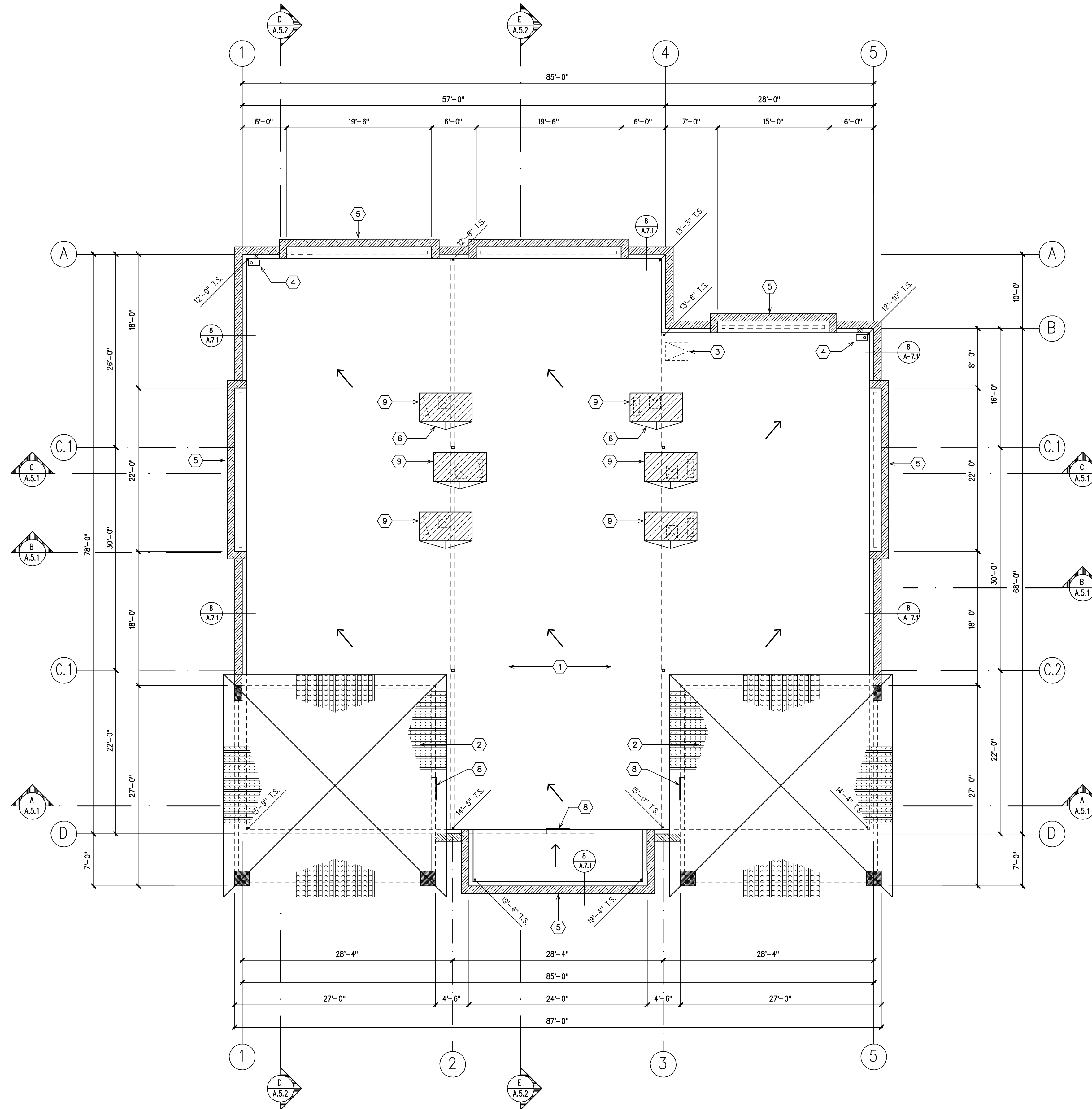
ROOF PLAN
